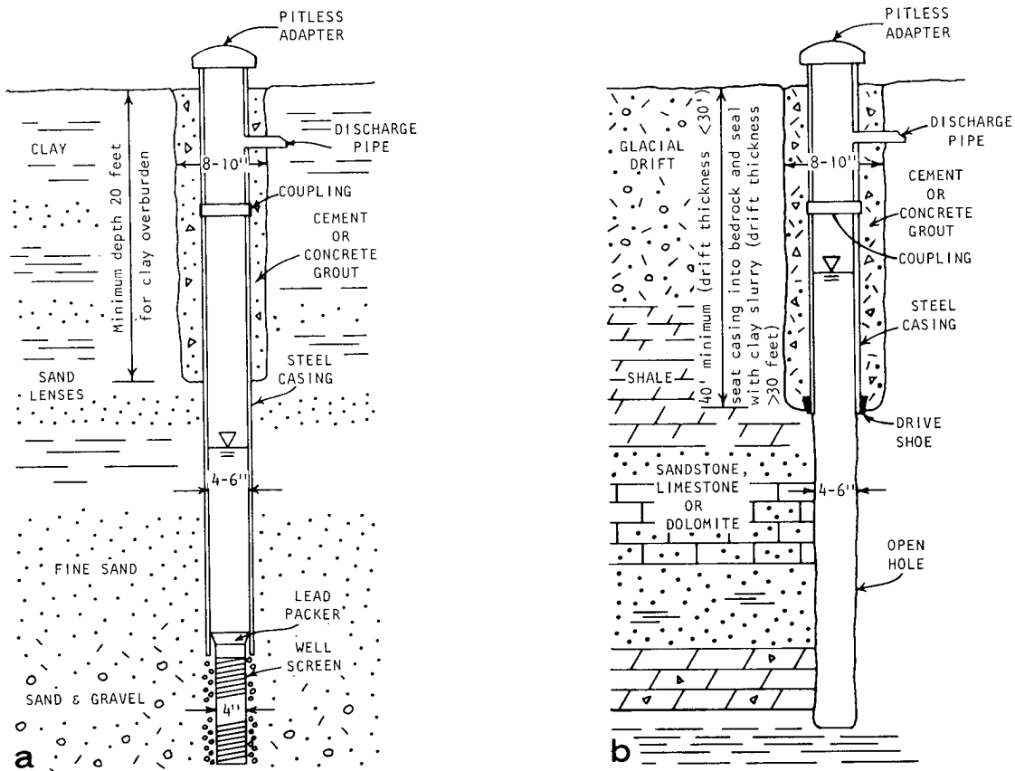
Figure 3. Typical domestic sand and gravel well (a) and bedrock well (b)
